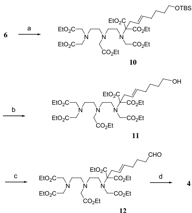
Scheme 3. Reagents and conditions: (a) 7 , \text{Pd}(\text{dba})_2 , dppe, THF, reflux; (b) TBAF, THF; (c) \text{SO}_3 :pyridine, TEA, DMSO; (d) \text{NaClO}_2 , \text{NaH}_2\text{PO}_4 , 2-methyl-2-butene, THF– t -BuOH– \text{H}_2\text{O} .
