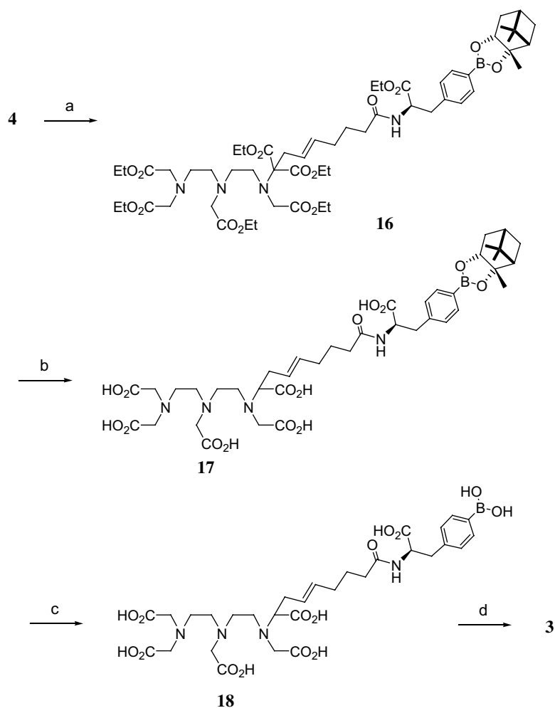
Scheme 4. Reagents and conditions: (a) 15 , DCC, \text{CH}_2\text{Cl}_2 , 0^\circ\text{C} ; (b) i. LiOH, \text{H}_2\text{O} ; ii. 10% HCl (pH ~ 2); (c) phenylboronic acid (2equiv) hexane- \text{H}_2\text{O} ; (d) \text{GdCl}_3 \cdot 6\text{H}_2\text{O} , \text{Na}_2\text{CO}_3 , \text{MeOH-H}_2\text{O} .
