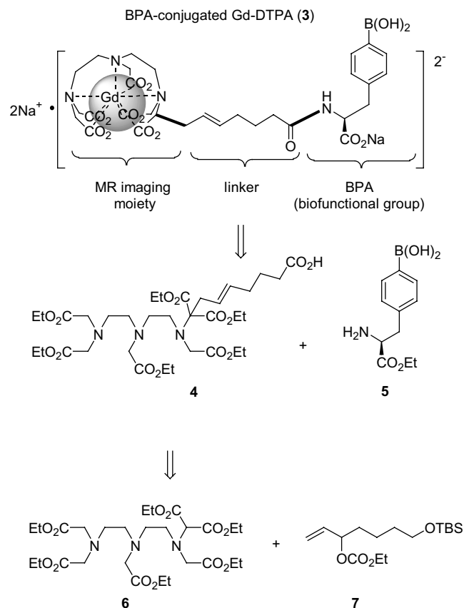
Scheme 1. Design of BPA-conjugated Gd–DTPA complex 3.
