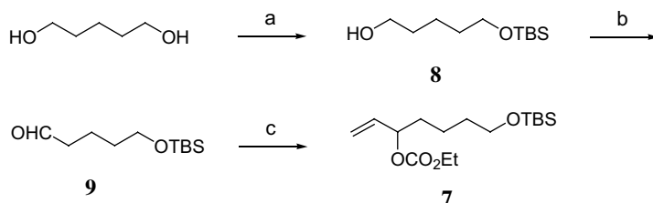
Scheme 2. Reagents and conditions: (a) i. TBSCl, imidazole, DMF, 0^\circ\text{C} ; (b) TEMPO, \text{NaClO} , \text{KBr} , \text{CH}_2\text{Cl}_2 – \text{H}_2\text{O} , 0^\circ\text{C} ; (c) i. vinyl magnesium bromide, THF, -78^\circ\text{C} ; ii. ethyl chloroformate.
